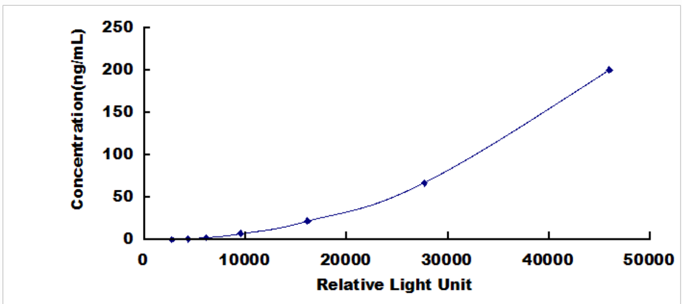
Typical Standard Curve for Trypsin, Porcine CLIA.
